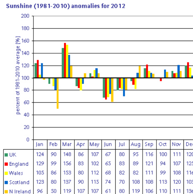
Figure 5: Sunshine (1981 – 2010) anomalies for 2012 (Met Office 2012)
