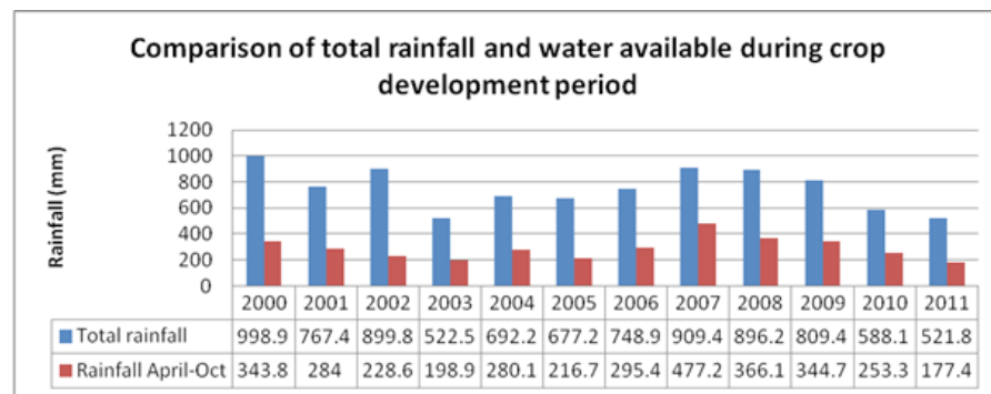
Figure 4: Variance between total rainfall and rainfall available during the growing period in Ross-on-Wye, Herefordshire (Met Office, 2012)
