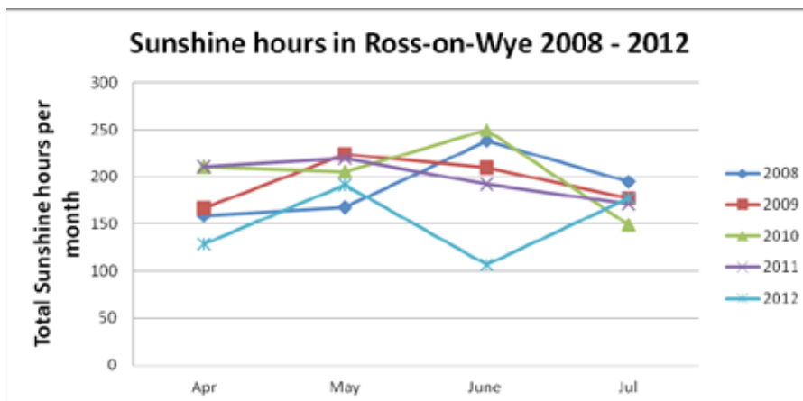
Figure 6: Sunshine hours recorded at Ross-on-Wye, Herefordshire between April and July 2008-2012 (Source of data: Met Office, 2012)
