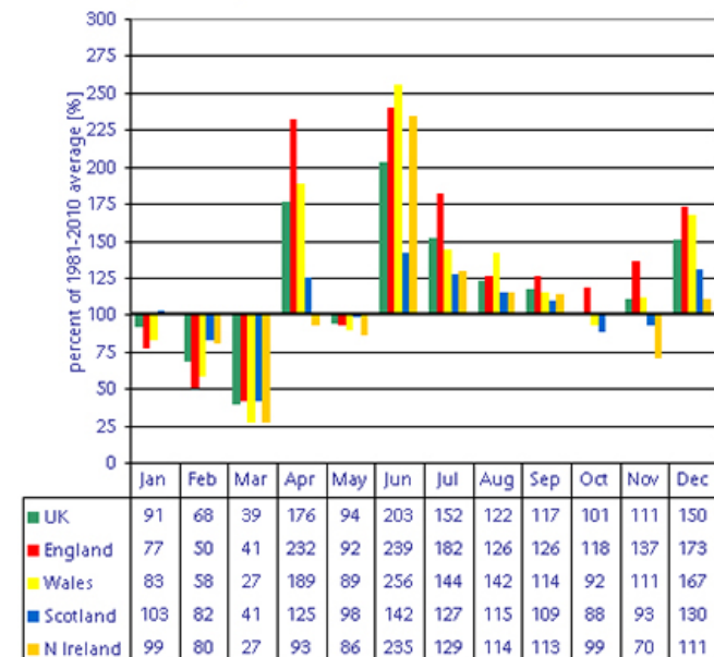
Figure 3: Rainfall (1981 – 2010) anomalies for 2012 (Met Office 2012)
